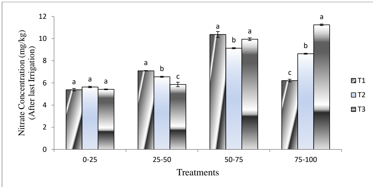
Figure 02. Effect of different tillage strategies on nitrate ( \text{NO}_3^- ) concentration in different depths of the soil after 6 th irrigation during maize ( Zea mays L. ) crop.
