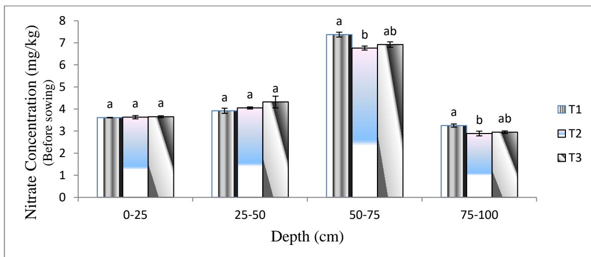
Figure 01. Effect of different tillage strategies on nitrate ( \text{NO}_3^- ) concentration in different depths of the soil before sowing of maize ( Zea mays L.) crop.
